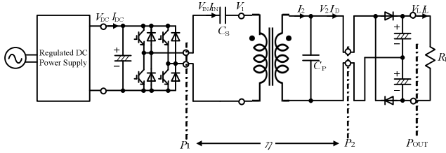
Figure 2. Contactless power transfer system.
